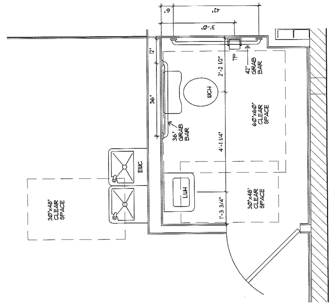
ENLARGED PLAN SCALE: 1/2" = 1'-0"
